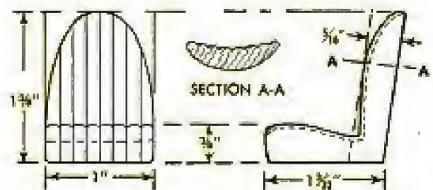
BUCKET SEATS, 2 REQD.
